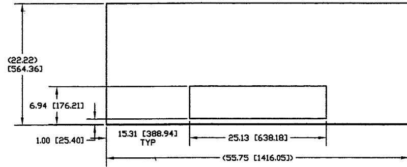
BOTTOM SHOE DOOR, CUTOUT DETAIL, 1/8 SCALE
