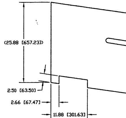
BOTTOM SHOE SIDES, CUTOUT DETAIL 1/8 SCALE
