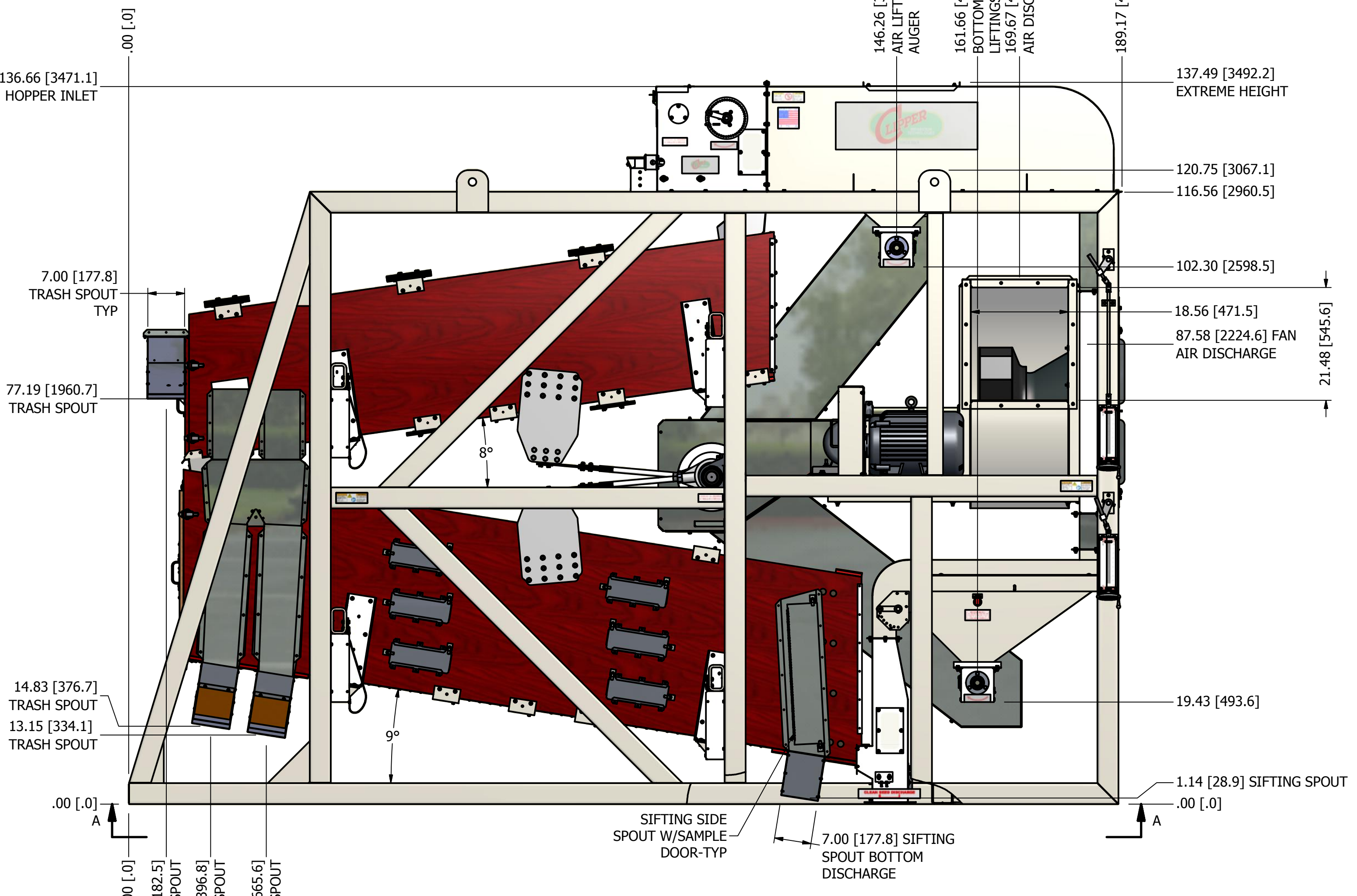
RIGHT SIDE VIEW RIGHT HAND DISCHARGE
