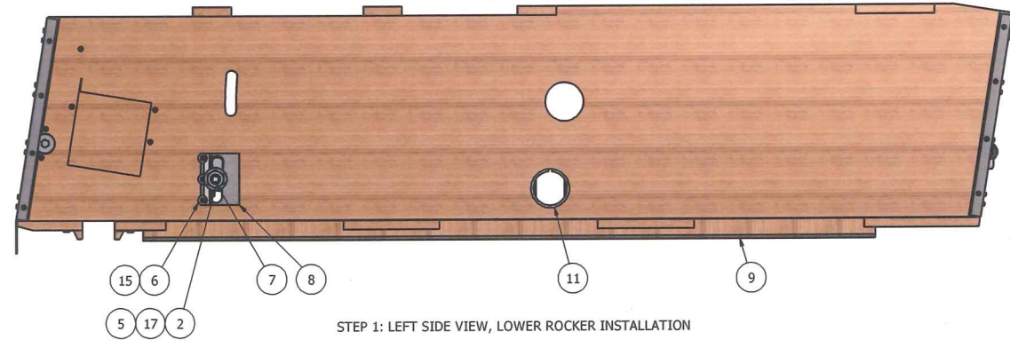
STEP 1: LEFT SIDE VIEW, LOWER ROCKER INSTALLATION
