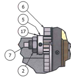
DETAIL D SCALE 0.38 : 1
