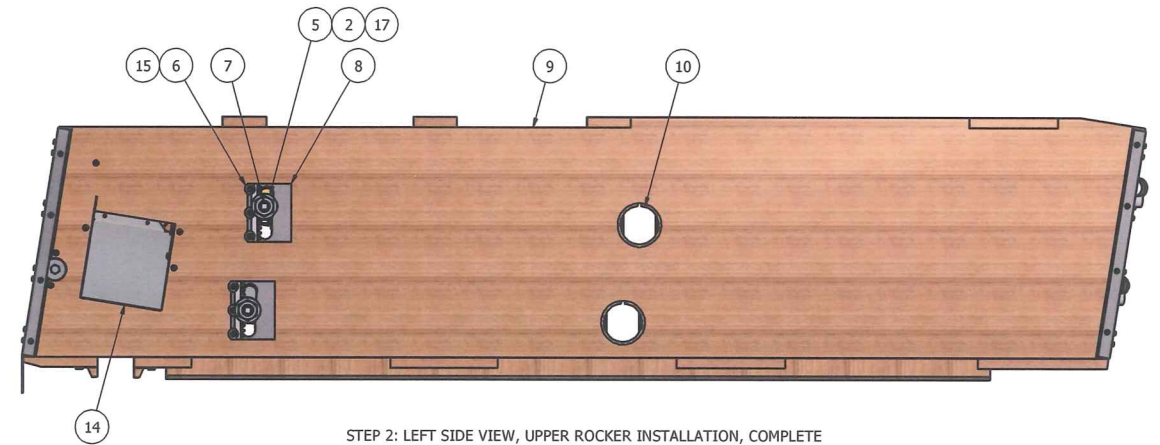
STEP 2: LEFT SIDE VIEW, UPPER ROCKER INSTALLATION, COMPLETE
