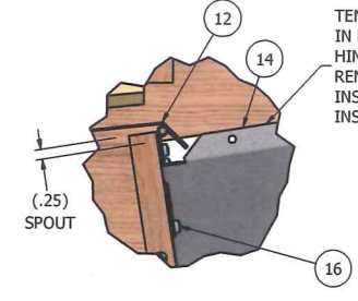
DETAIL F SCALE 0.38 : 1
