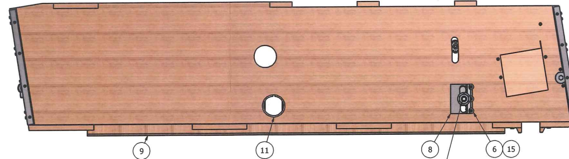
STEP 1: RIGHT SIDE VIEW, BOTTOM ROCKER INSTALLATION
