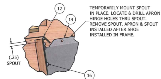
DETAIL F SCALE 0.38 : 1
