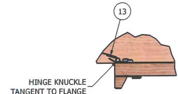
DETAIL C SCALE .38:1
