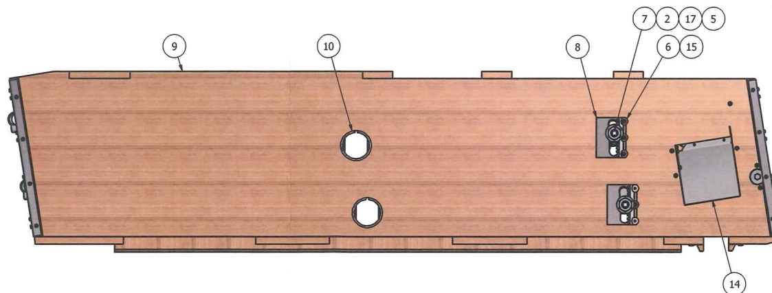
STEP 2: RIGHT SIDE VIEW, UPPER ROCKER INSTALLATION
