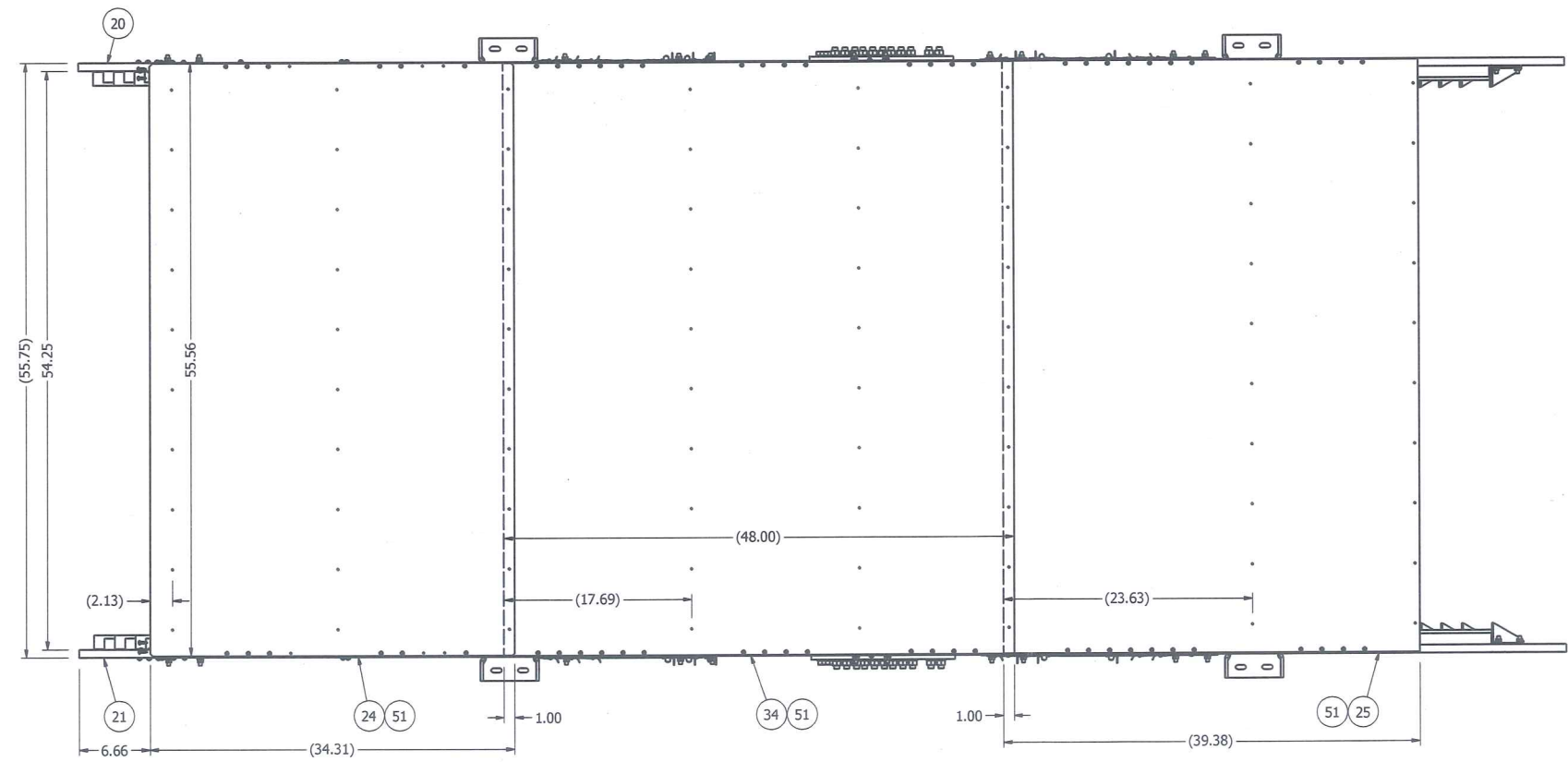
BOTTOM VIEW - BOTTOM METAL ASSY
