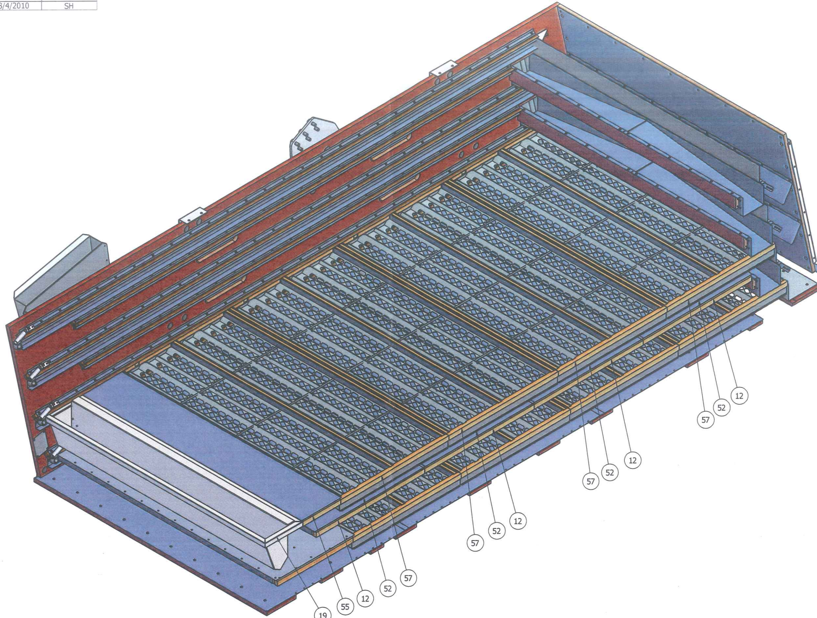
SCREEN, BALL & BLANK RAIL INSTALL 3RD RAIL SHOWN
