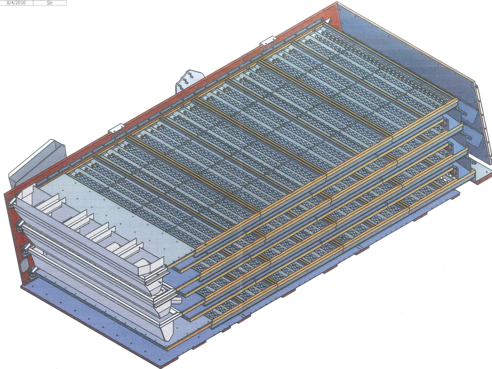
SCREEN, BALL & BLANK RAIL INSTALL 1ST RAIL SHOWN
