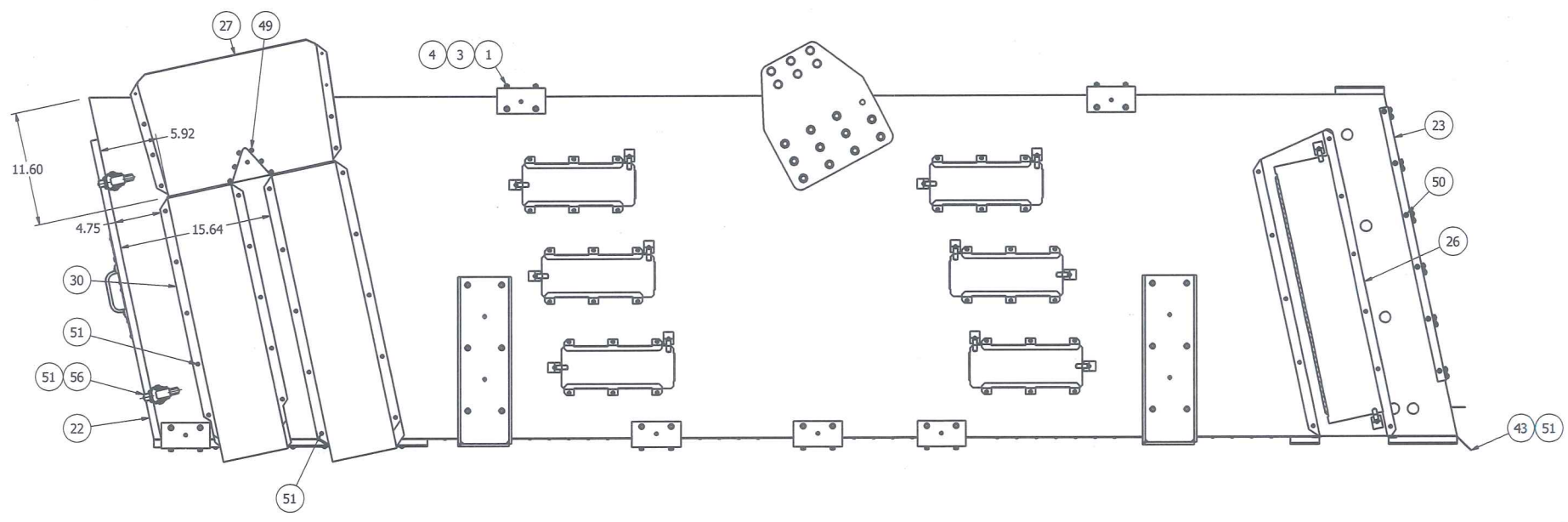
RIGHT SIDE - EXTERNAL ASSY
