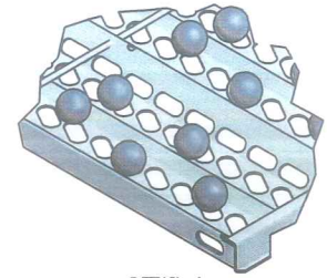
DETAIL A SCALE 1 / 4 5 BALLS (F80026101) PER COMPARTMENT 80 BALLS PER TRAY
