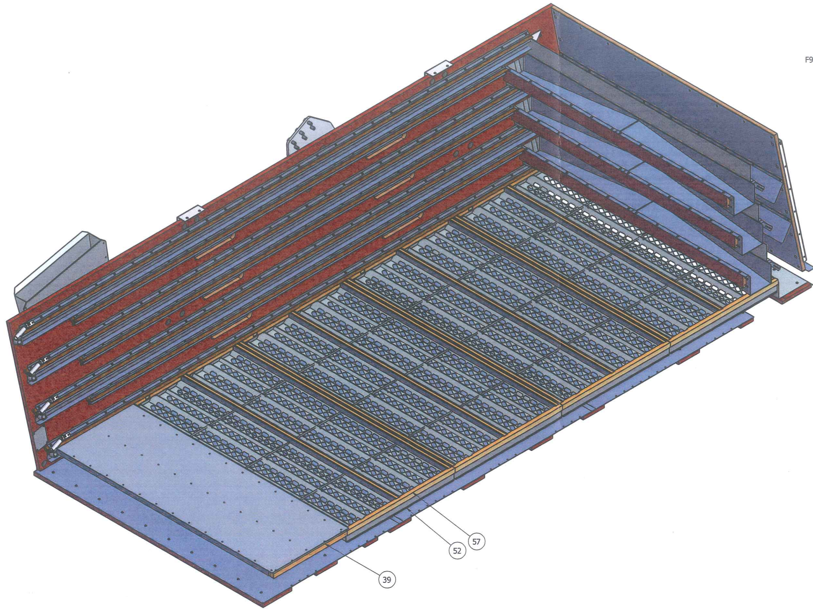
SCREEN & BALL TRAY INSTALL 4TH RAIL SHOWN
