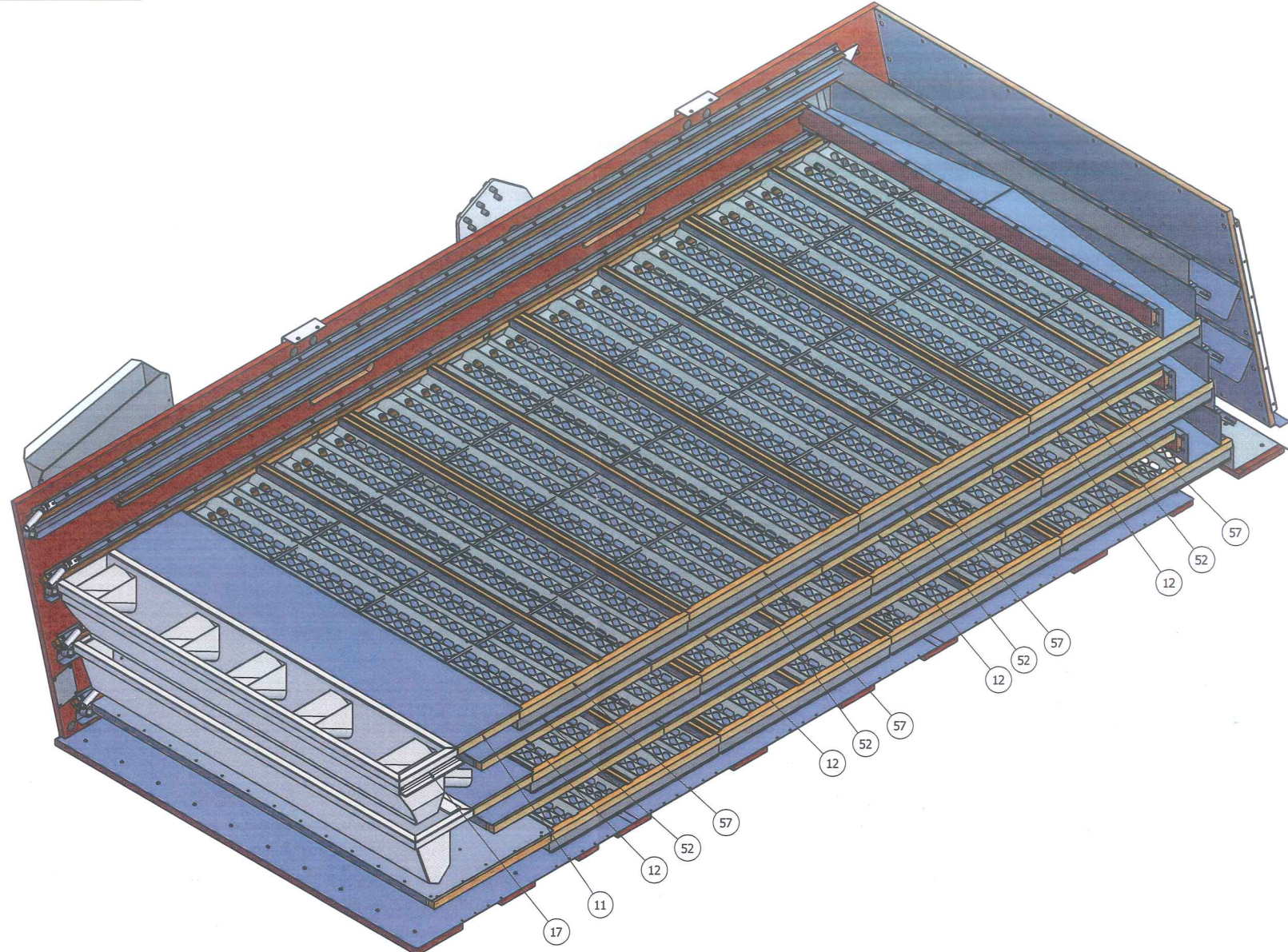
SCREEN, BALL & BLANK RAIL INSTALL 2ND RAIL SHOWN
