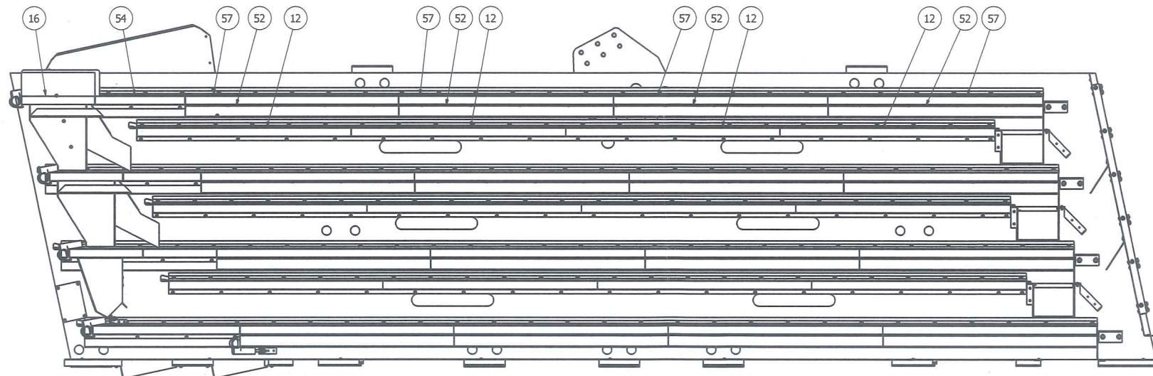
SCREEN, BALL & BLANK RAIL INSTALL 1ST RAIL SHOWN
